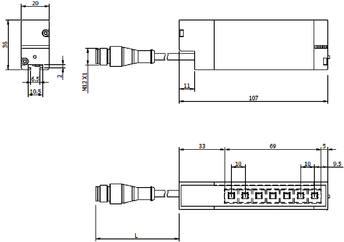
Pict.: 1 Pigtail cable length L= 240mm
